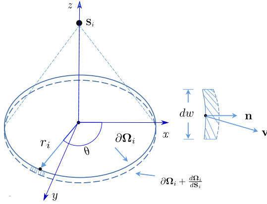
Fig. 2. Illustration of the gradient on the boundary.
