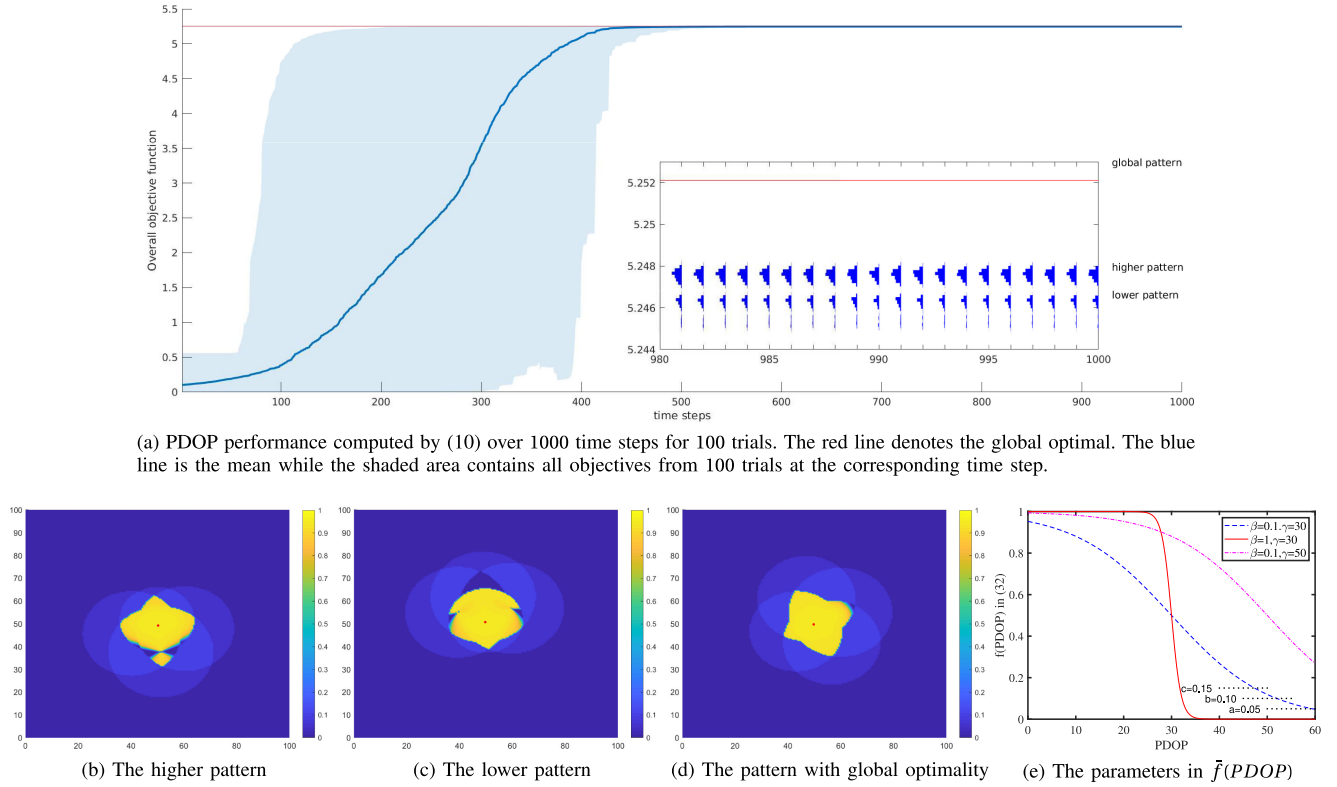
Fig. 3. Statistical results for four robots serving a fixed density. (b,c,d) are the distributions of \bar{f}(\cdot) for each pattern. Red dots are the maximum point.
