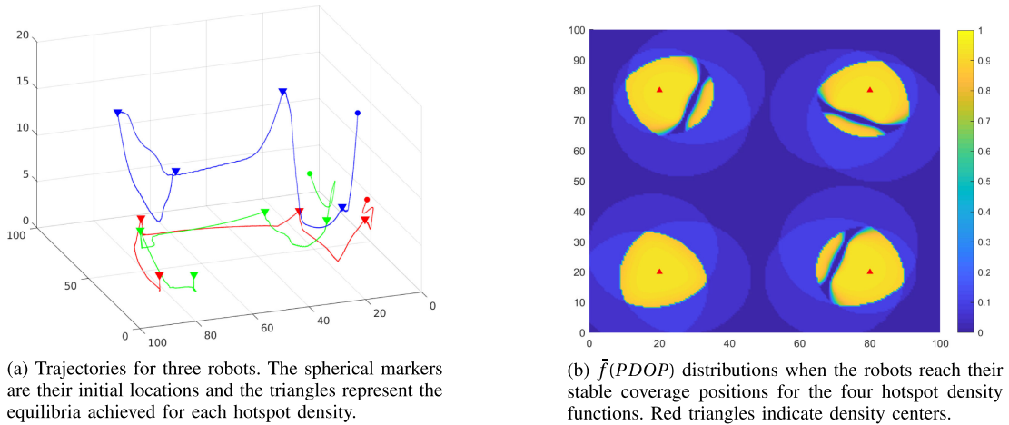
Fig. 5. Simulation results for the time-varying hotspot densities over 2000 steps, whose centers are switched every 500 steps. The sequence of centers is d_{c1} = [20, 20]^T , d_{c2} = [80, 20]^T , d_{c3} = [80, 80]^T , d_{c4} = [20, 80]^T . These centers are also the points with maximum \hat{f}(\cdot) values.
